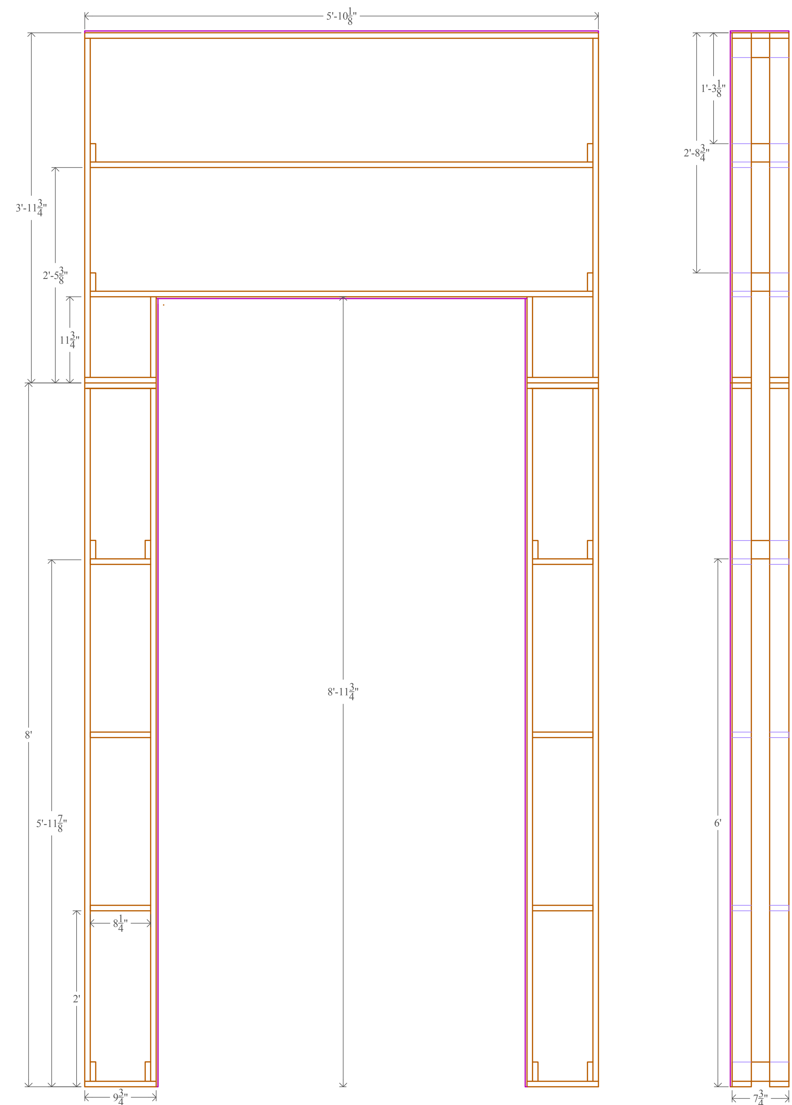
Door B Framing Scale: 1 1/2" = 1'- 0" Build 1
