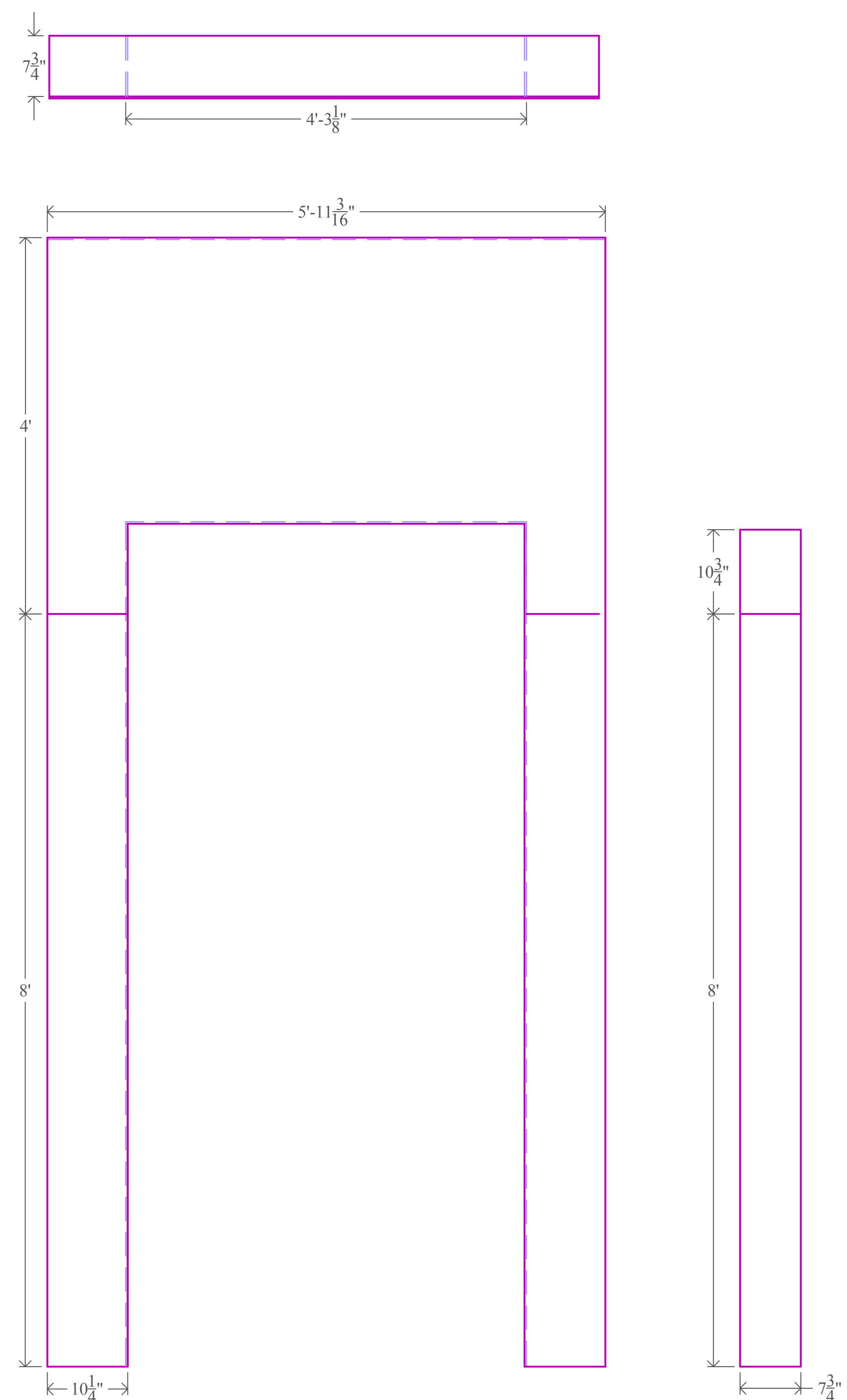
Door B Framing Scale: 1" = 1'- 0" Build 1
