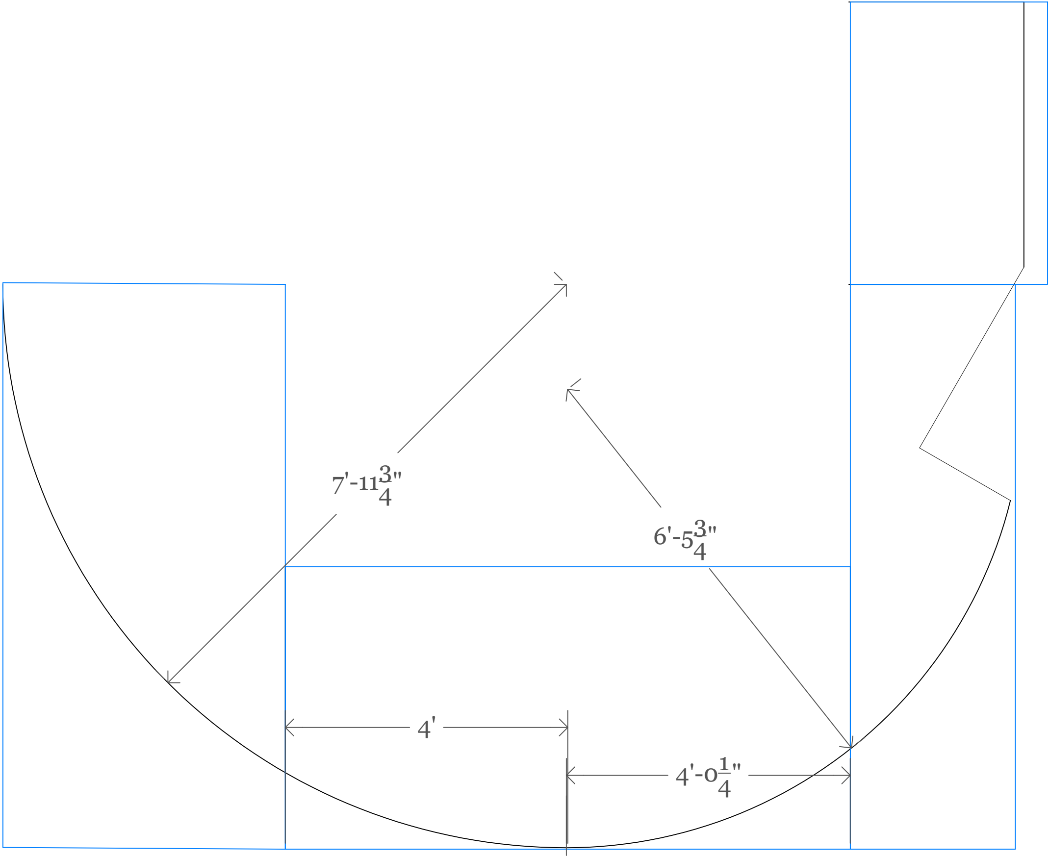
Flapjack Platforms - Facing Layout Top View
