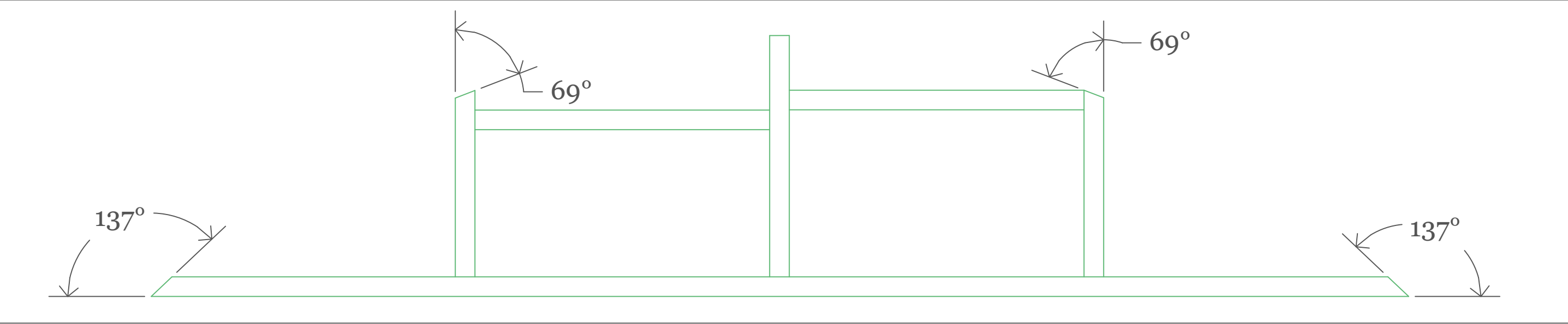
Pie Platforms - P2 Framing Angles Top View Build 1 Scale 1 1/2" = 1'-0"
