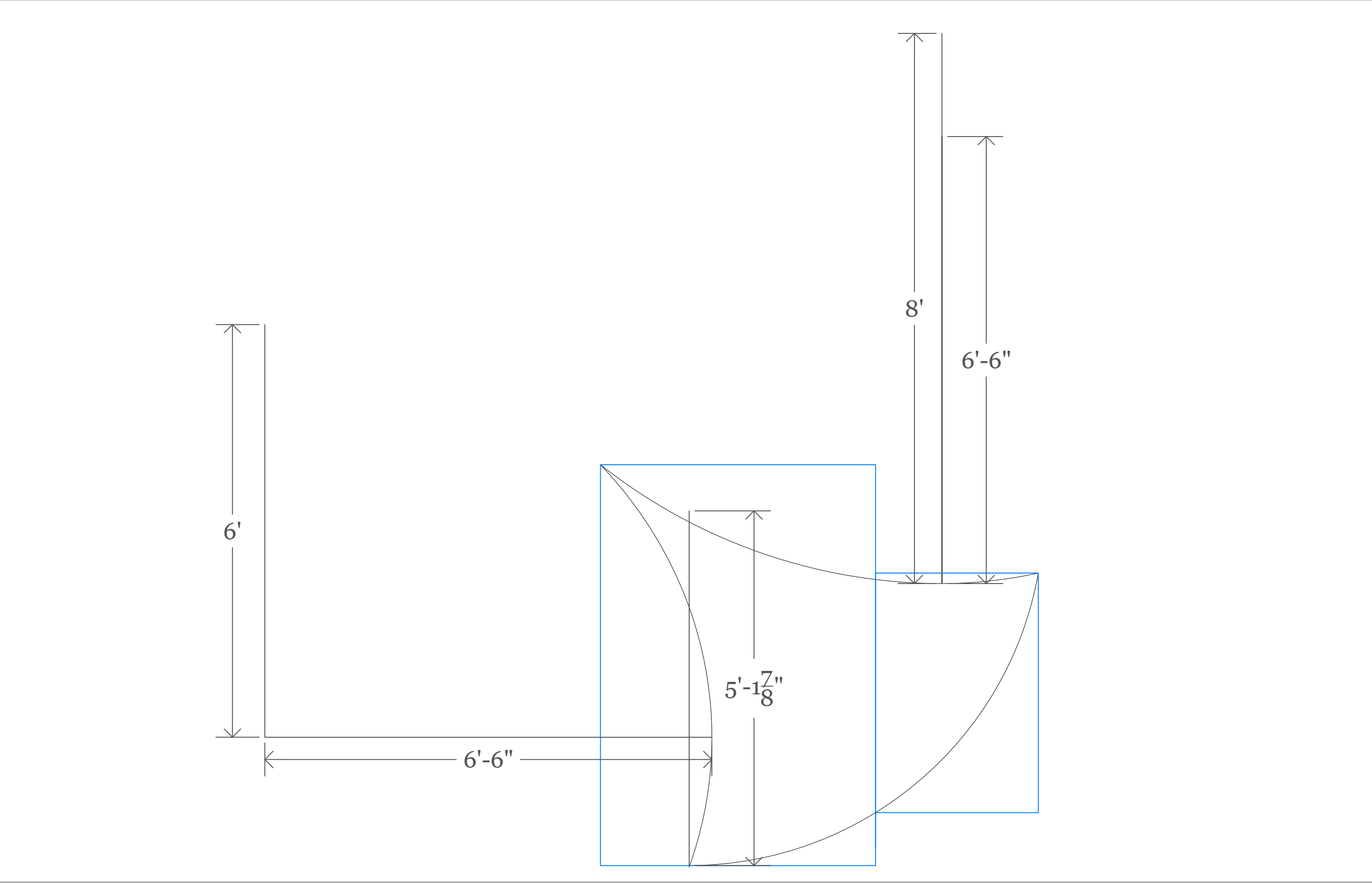
Jerry Platform - OSB Lid Jig Rips Top View Rip 1 Scale 1" = 1'-0"
