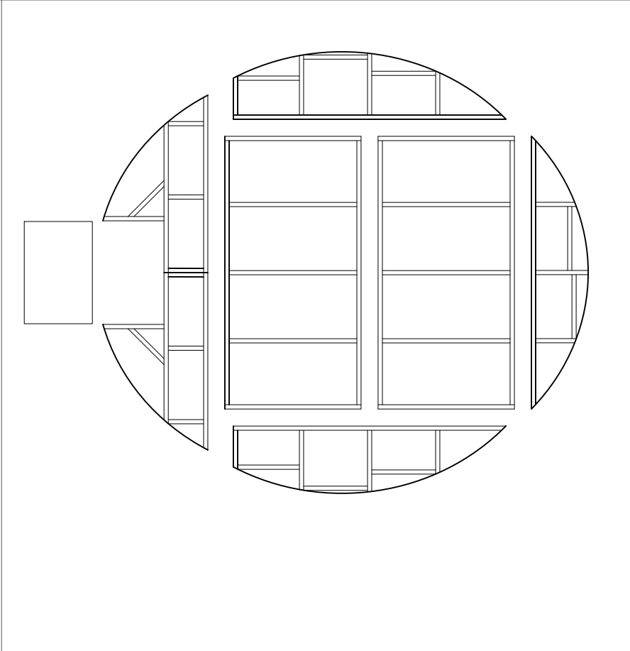
Pie Platforms - Exploded Framing Top View Scale 1/4" = 1'-0"
