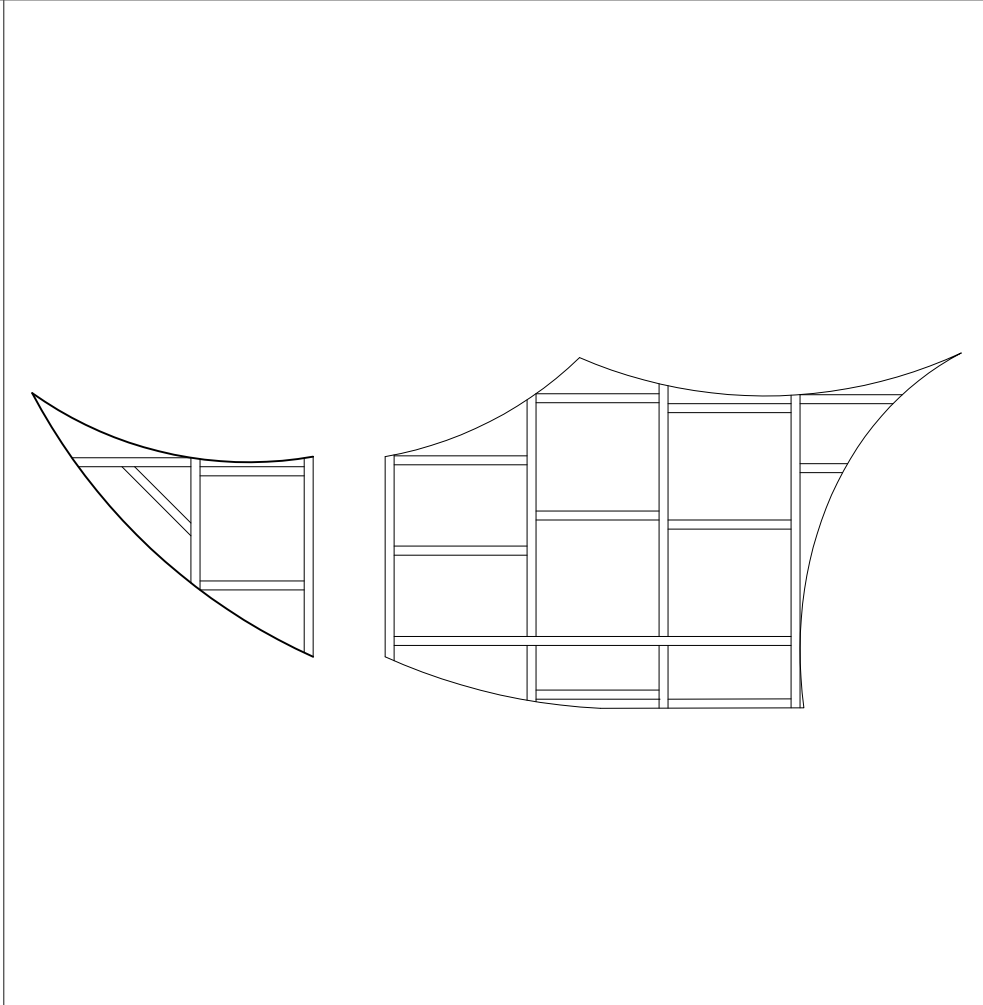
Geri Platforms - Exploded View Top View Build 1 Scale 3/8" = 1'-0"
