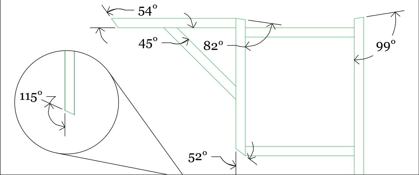
Geri Platforms - G2 Framing Angles Top View Build 1 Scale 1 1/2" = 1'-0"
