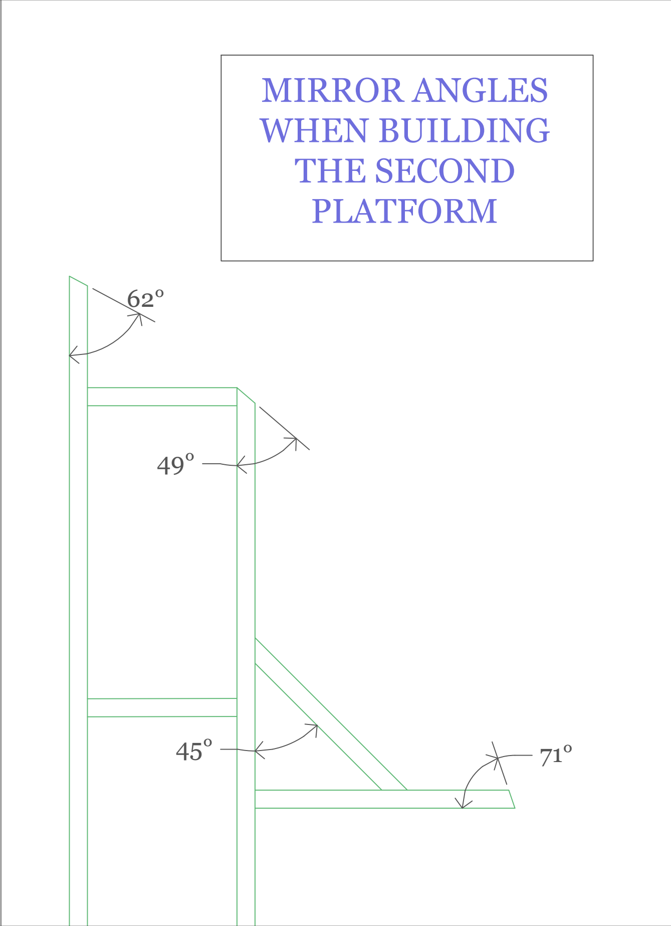
Pie Platforms - P4 & P5 Framing Angles Top View
