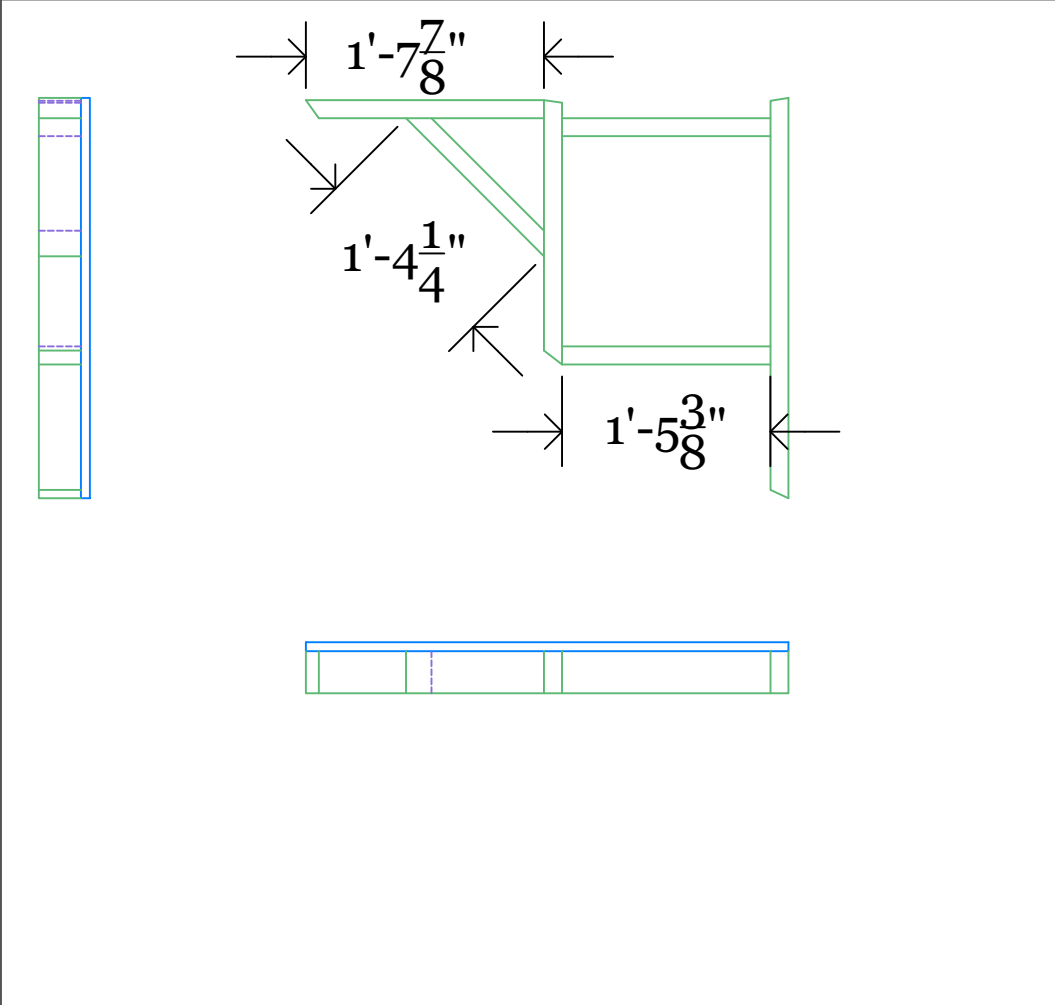
Geri Platforms - G2 Framing Top View Build 1 Scale 3/4" = 1'-0"
