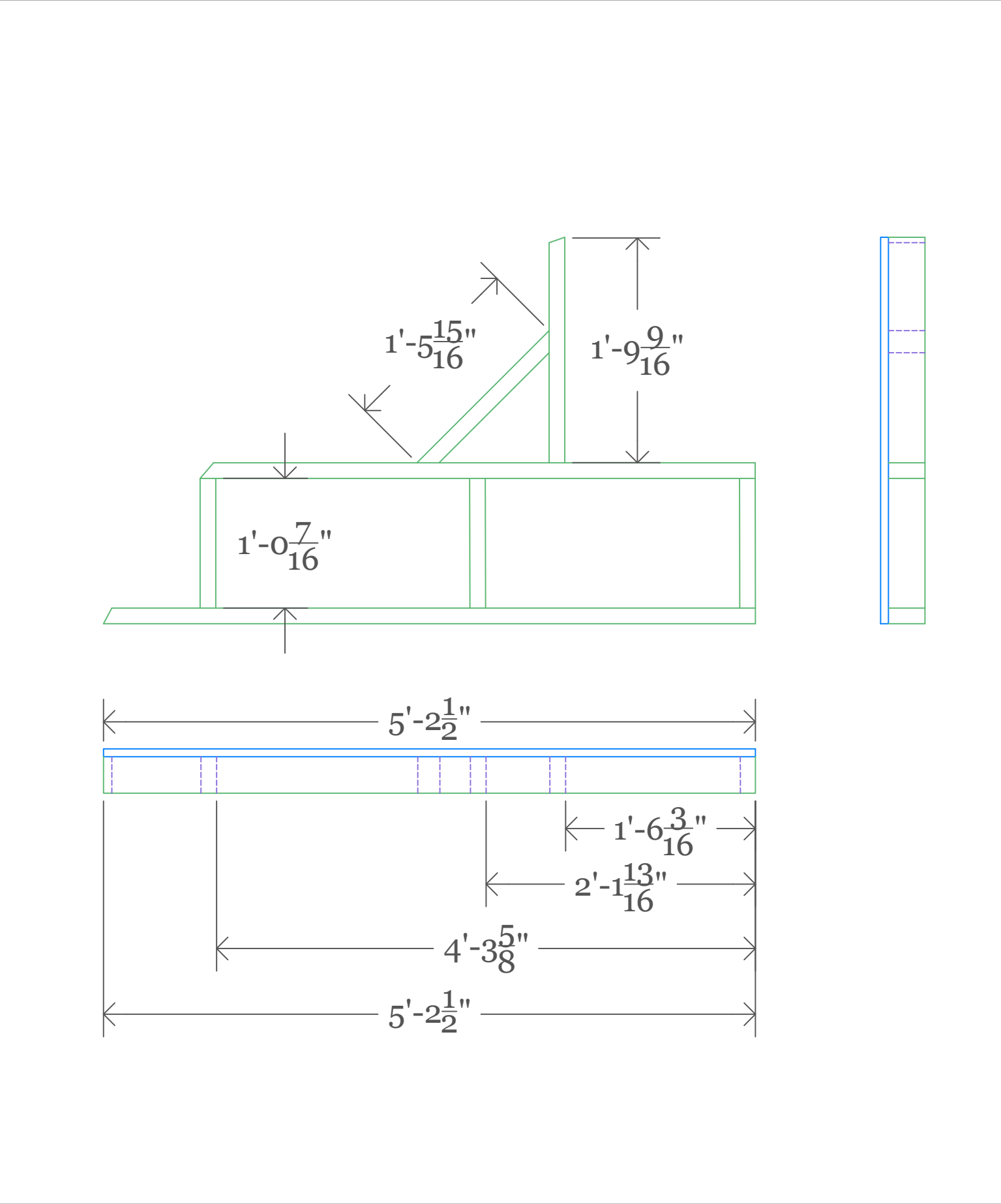
Pie Platforms - P4 & P5 Framing Top View
