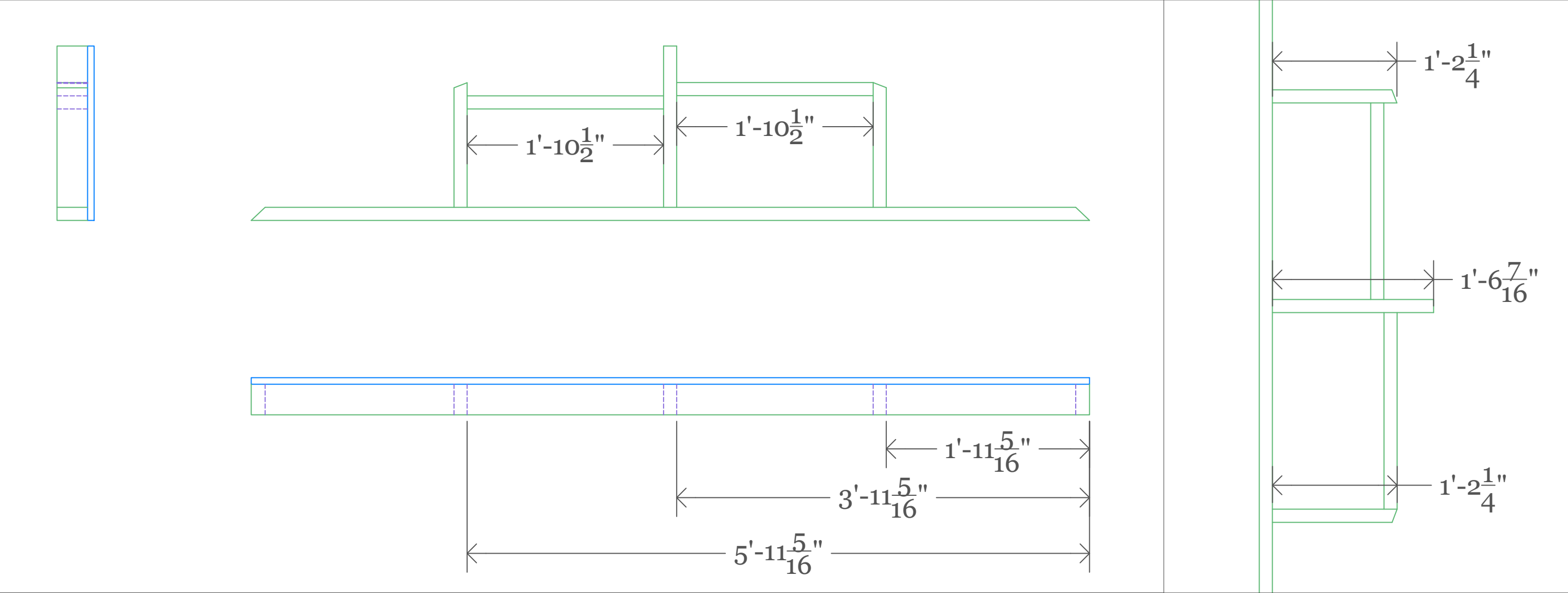
Pie Platforms - P2 Framing Top View Build 1 Scale 1" = 1'-0"
