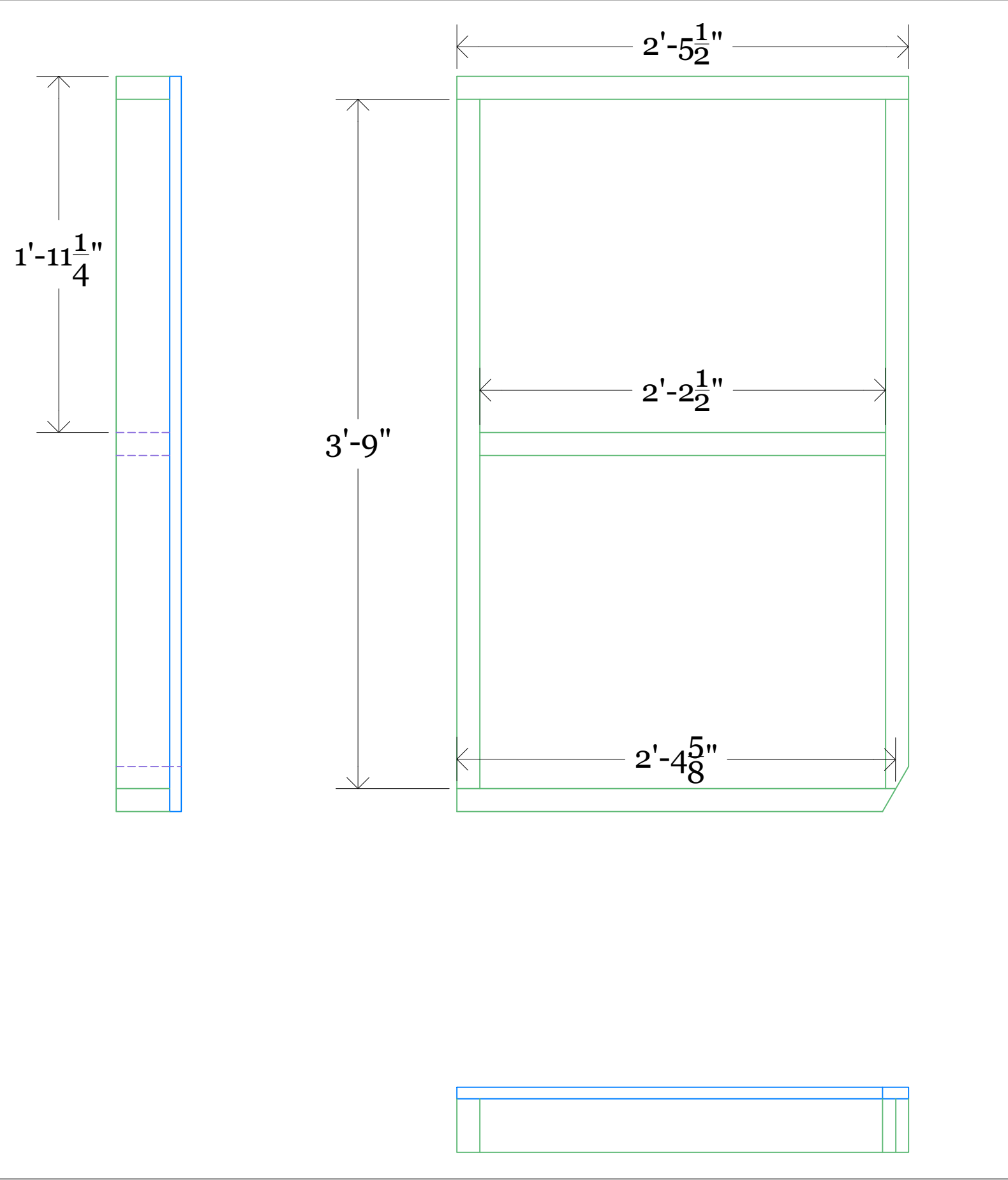
Flapjack Platforms - F3 Framing Top View
