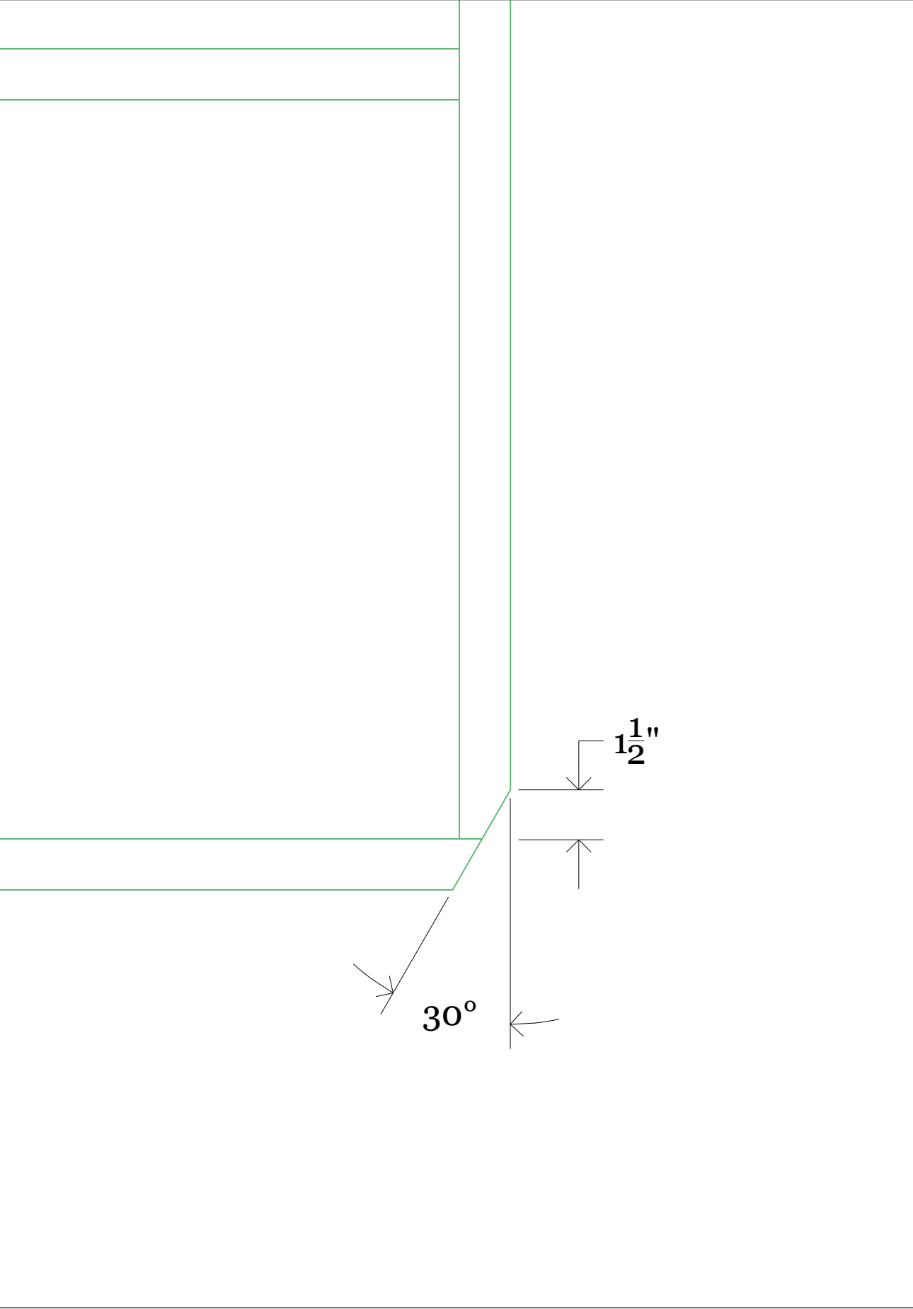
Flapjack Platforms - F3 Framing Angles Top View
